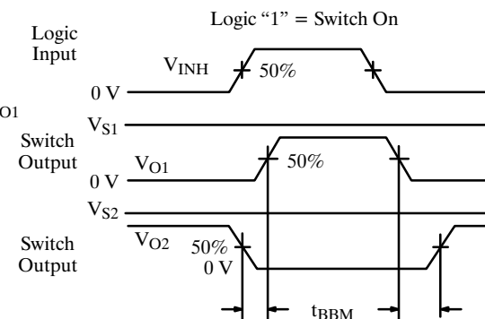
Figure 2. Switching Time
