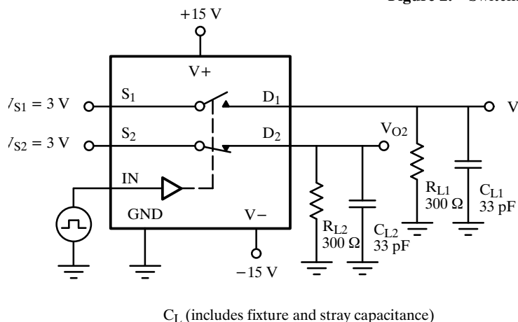
Figure 3. Break-Before-Make SPDT (DG301A, DG303A)
